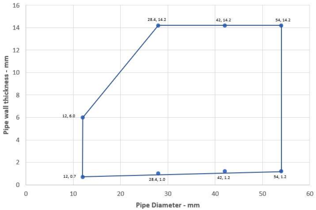
Copper or Steel Pipes 12-54 / Insulated - C/C
